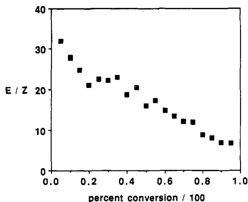
Figure 1. Selectivity of 3-pentanone enolization according to eq 1. E/Z = [6]/[7] . Enolization was effected at -78^\circ\text{C} with 0.1 M LiTMP in THF.
