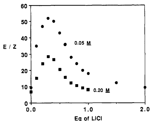
Figure 2. Selectivity of 3-pentanone enolization according to eq 1. E/Z = [6]/[7] . Enolization was run to 77% conversion at -78^\circ\text{C} by LiTMP (at concentrations indicated) with varying amounts of added LiCl in THF.
