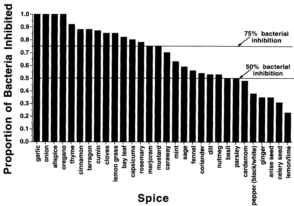
FIGURE 6. ANTIMICROBIAL PROPERTIES (INHIBITION OF GROWTH OR KILLING) OF 30 SPICES FOR WHICH APPROPRIATE DATA WERE AVAILABLE (SEE APPENDIX A), ARRAYED FROM GREATEST TO LEAST INHIBITION. All spices inhibit some species of food-spoilage bacteria they have been tested on, and about half inhibit \geq 75\% of bacteria.
