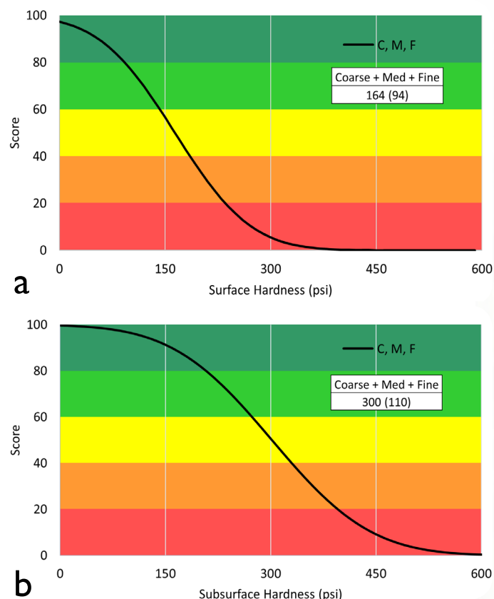
FIGURE 4 a and b. Surface (a) and subsurface (b) scoring functions and upper value limits for Coarse(C), Medium (M) and Fine (F) textural classes.
