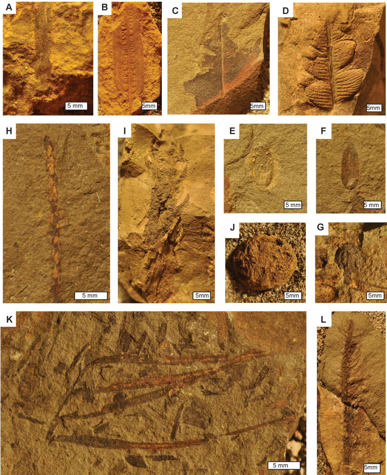
Fig. 9. Fossil plant impressions: horsetail Equisetites burchardtii (A), fern Nathorstia angustifolia (B), cycadeoid Nilssonia canadensis (C), cycadeoid Nilssonia schaumbergensis (D), Cycadeospermum lineatum (E-F), two seeded conifer cone unit (G), conifer shoot Cyparissidium gracile (H), conifer shoot and cone Elatides splendida (I, J), conifer shoot Elatocladus smittiana (K), conifer shoot Margeriella cretacea (L). Specimen numbers are F127880 (A), F120569 (B), F127957A (C), F127956 (D), F127982 (E), F127983E (F), F127961 (G), F127967 (H), F127963 (I), F127975 (J), F127072 (K), F127885A (L).
