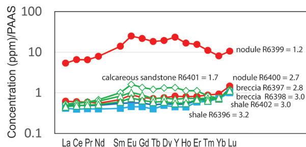
Fig. 6. YREE patterns normalized to Post-Archaean Australian Shale of the green breccia and contained nodules compared with shales of the Hudspeth Formation above and below.
