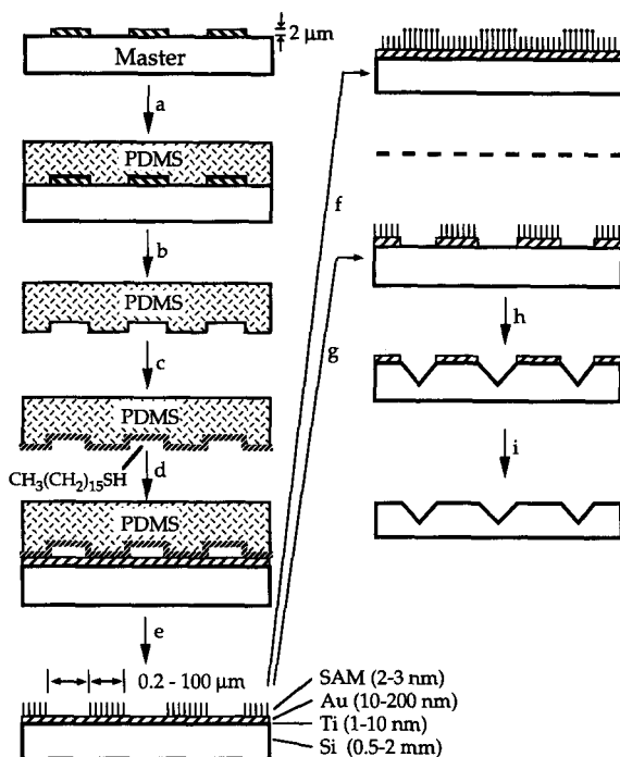
Figure 5 Microcontact printing starts with a master template containing a pattern of relief (a); this master can be fabricated by photolithography or by other methods. A PDMS stamp cast from this master (b) is inked with a solution of alkanethiol in ethanol (c) and used to transfer the alkanethiol to surface of gold (d); a SAM is formed only at those regions where the stamp contacts the surface (e). The bare regions of gold can then be derivatized with a different SAM by rinsing with a solution of a second alkanethiol (f). The initial patterned SAM can also be used to protect the underlying gold from dissolution in a corrosive etchant (g). Anisotropic etching of the exposed silicon gives contoured surfaces (h). The gold mask can be removed by washing with aqua regia ; the resulting silicon substrates are useful as new masters from which stamps can be cast or as substrates for a variety of applications.
