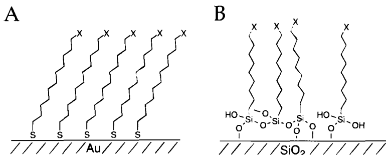
Figure 2 Models for SAMs of alkanethiolates on gold and alkylsiloxanes on hydroxylated surfaces. (A) The thiol groups coordinate to the hollow threefold sites of the gold (111) surface, and the alkyl chains pack in a quasi-crystalline array. (B) The conformations of alkylsilanes and the details of their bonding to surface hydroxyl groups are less clear; a mixture of possible conformations and geometries is probably involved. The surface properties of both SAMs are controlled by controlling the terminal function group X.
