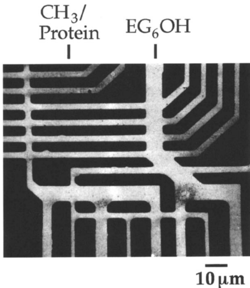
Figure 6 Scanning electron micrograph of fibrinogen adsorbed on a patterned SAM. A patterned hexadecanethiolate SAM on gold was formed by \mu CP, and the remainder of the surface was derivatized by immersion in a solution containing a hexa(ethylene glycol)-terminated alkanethiol [ \text{HS}(\text{CH}_2)_{11}(\text{OCH}_2\text{CH}_2)_6\text{OH} ]. The patterned substrate was immersed in a solution of fibrinogen (1 mg/mL) in phosphate-buffered saline for 2 h, removed from solution, rinsed with water, and dried. Fibrinogen adsorbed only to the methyl-terminated regions of the SAM, as illustrated by the dark regions in the micrograph: Secondary electron emission from the underlying gold is attenuated by the protein adlayer.
