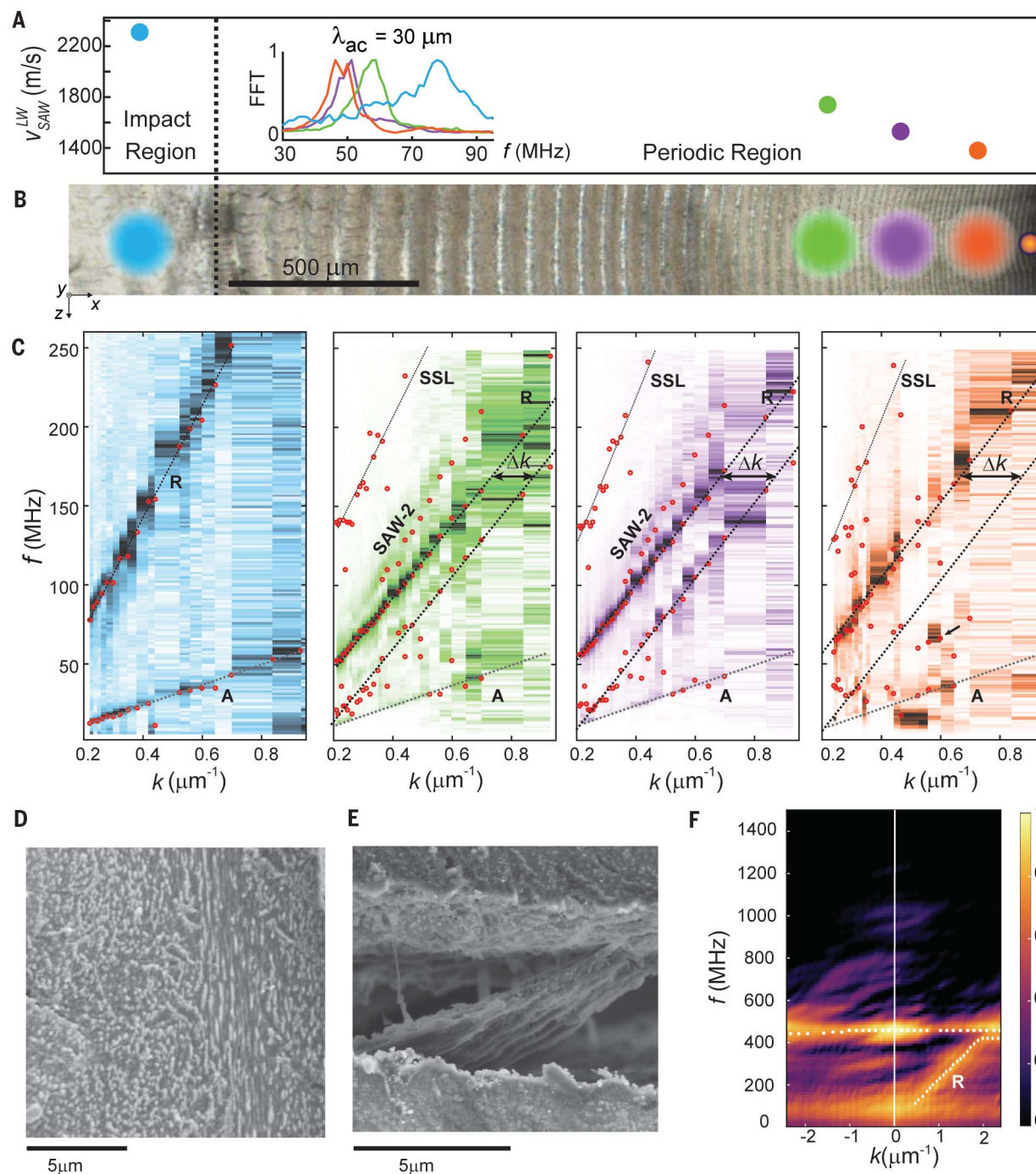
Fig. 2. Ultrasonic phononic dispersion of the mantis shrimp's dactyl club. (A) Frequency ( f ) spectrogram obtained by fast Fourier transform (FFT) and phase speed variation in the impact and periodic regions obtained by TGS at an acoustic wavelength ( \lambda_{ac} = 30 \mu\text{m} ). (B) Enlarged view of the cross section of the dactyl club with regions probed by TGS (large spot sizes) and PLU (small spot size); the colored regions illustrate the position and sizes of the probed regions.
