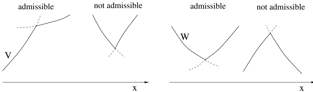
Figure 34: Left: the value function V for a minimization problem. Right: the value function W for a maximization problem.
