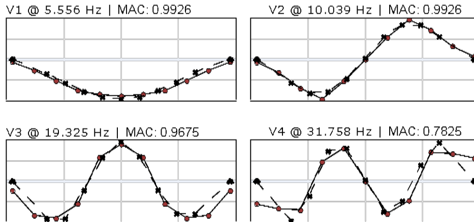
Figure 6: Vertical mode shapes.
