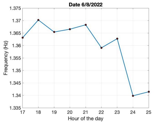
Figure 5: Mode 2 frequency (~1.3) throughout the day on 6/8/2022
