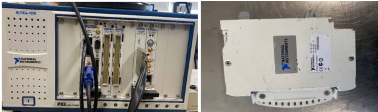
Figure 23. The NI DAQ system (NI PXIe-1078) and Data Acquisition Junction Box (NI TB-4330).
