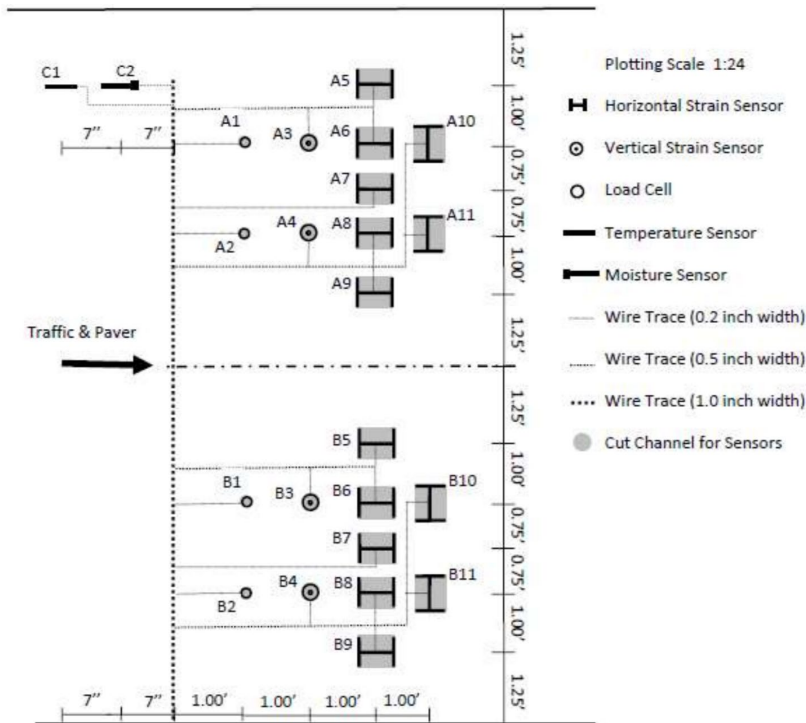
Figure 20. Sensor Distribution and Layout in a VDOT overlay project (Wang et al., 2012).
