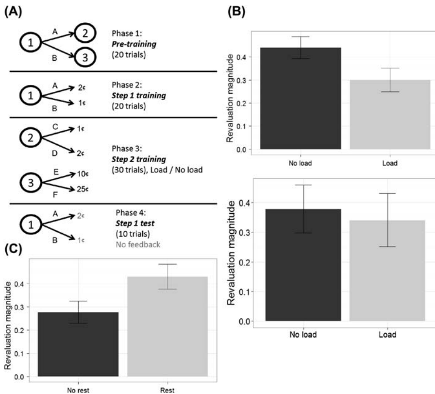
Figure 7.6 (A) The sequential decision problem consists of three states (indicated by numbered circles) and two mutually exclusive actions in each state (indicated by letters). Deterministic transitions between states conditional upon the chosen action are indicated by arrows. Rewards for each state–action pair are indicated by amounts (in cents). In Phase 4, reward feedback is delayed until the end of the phase. (B) Revaluation in load and no load conditions. Revaluation magnitude is measured as P_4(\text{action} = B | \text{state} = 1) - P_2(\text{action} = B | \text{state} = 1) , where P_i(\text{action} = a | \text{state} = s) is the probability of choosing action a in state s during Phase i . Top: load applied during Phase 3; Bottom: load applied during Phase 4. (C) A brief rest phase prior to Phase 4 ameliorates the effects of load.
