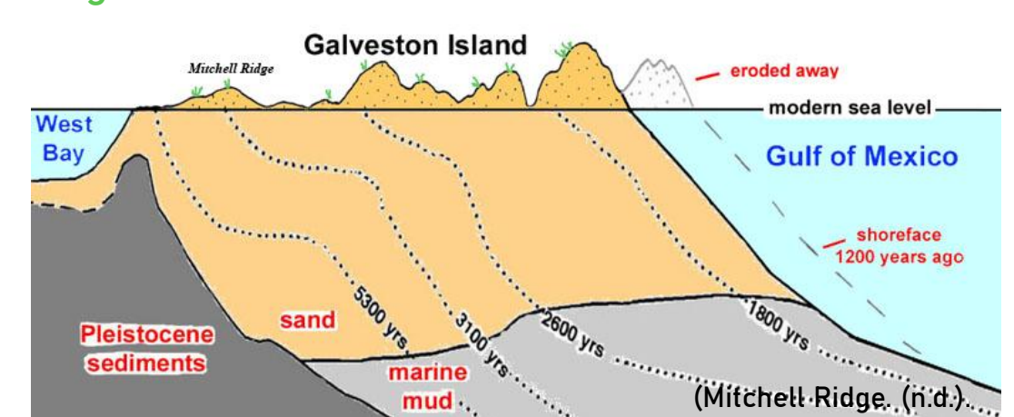
Figure 9. Galveston island depositional history. (Mitchell Ridge, R.D.)
