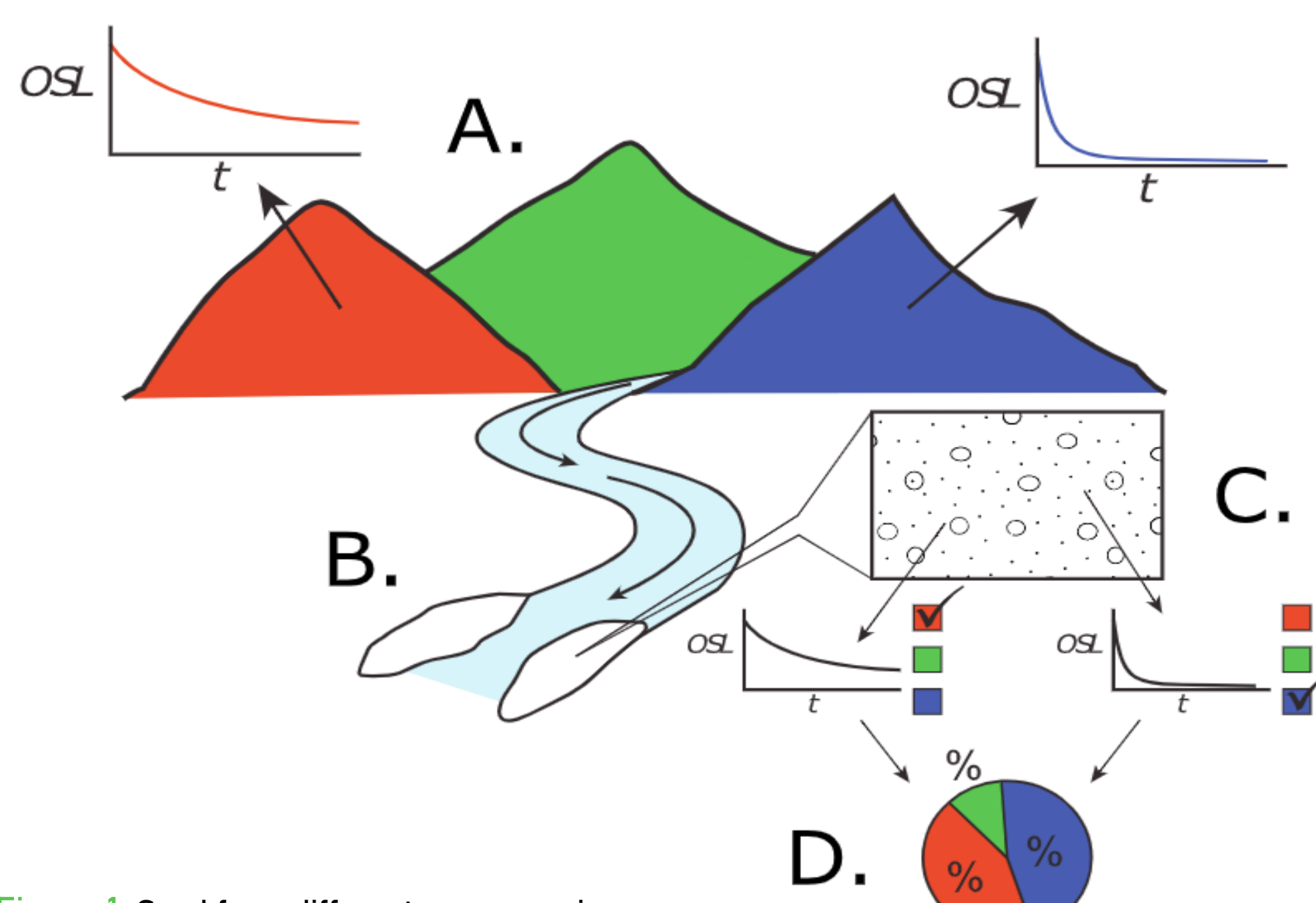
Figure 1. Sand from different source regions can have different luminescence sensitivities.
