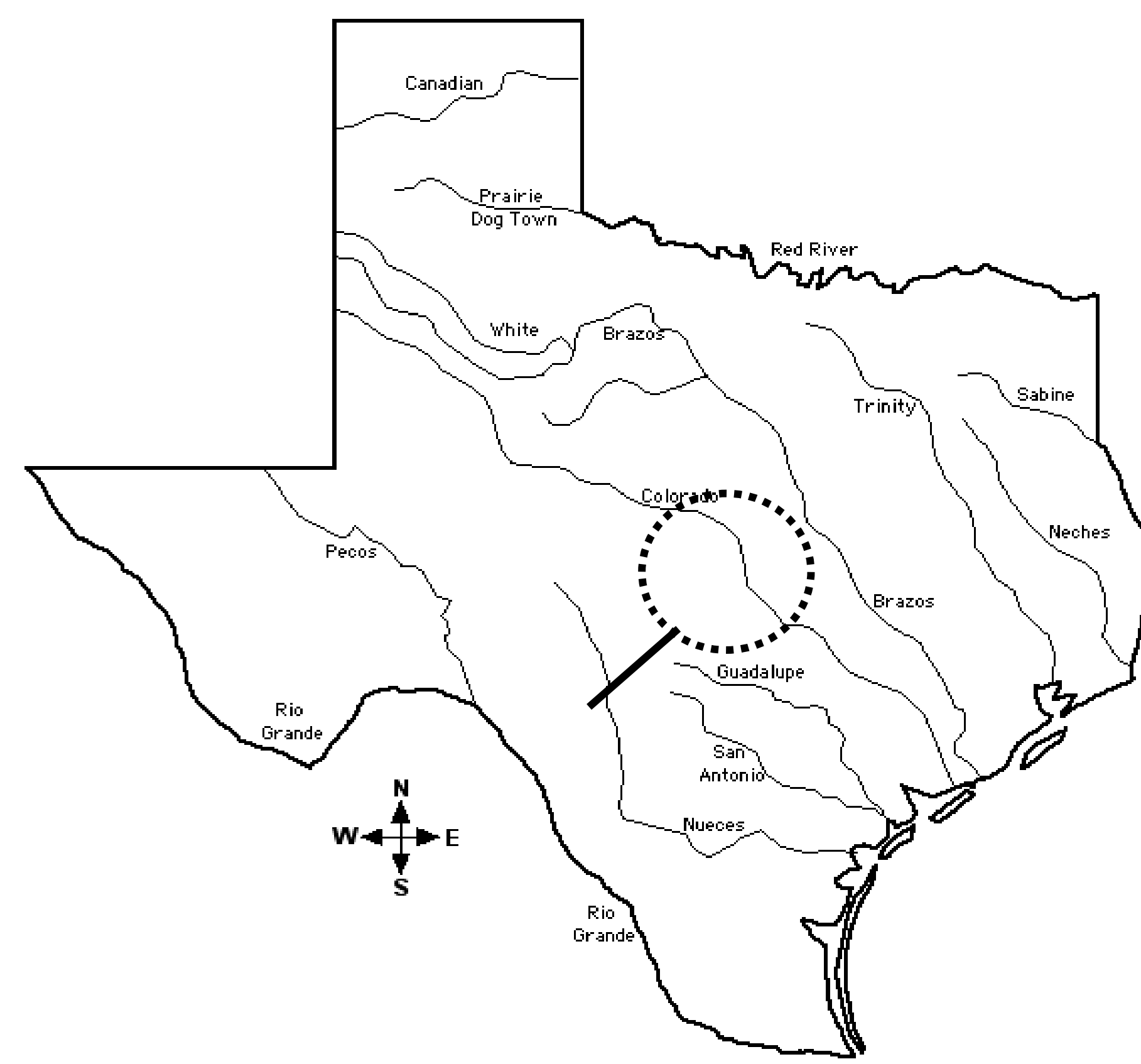
Figure 5. Major river systems in Texas with Llano Uplift region highlighted with magnifying glass.
