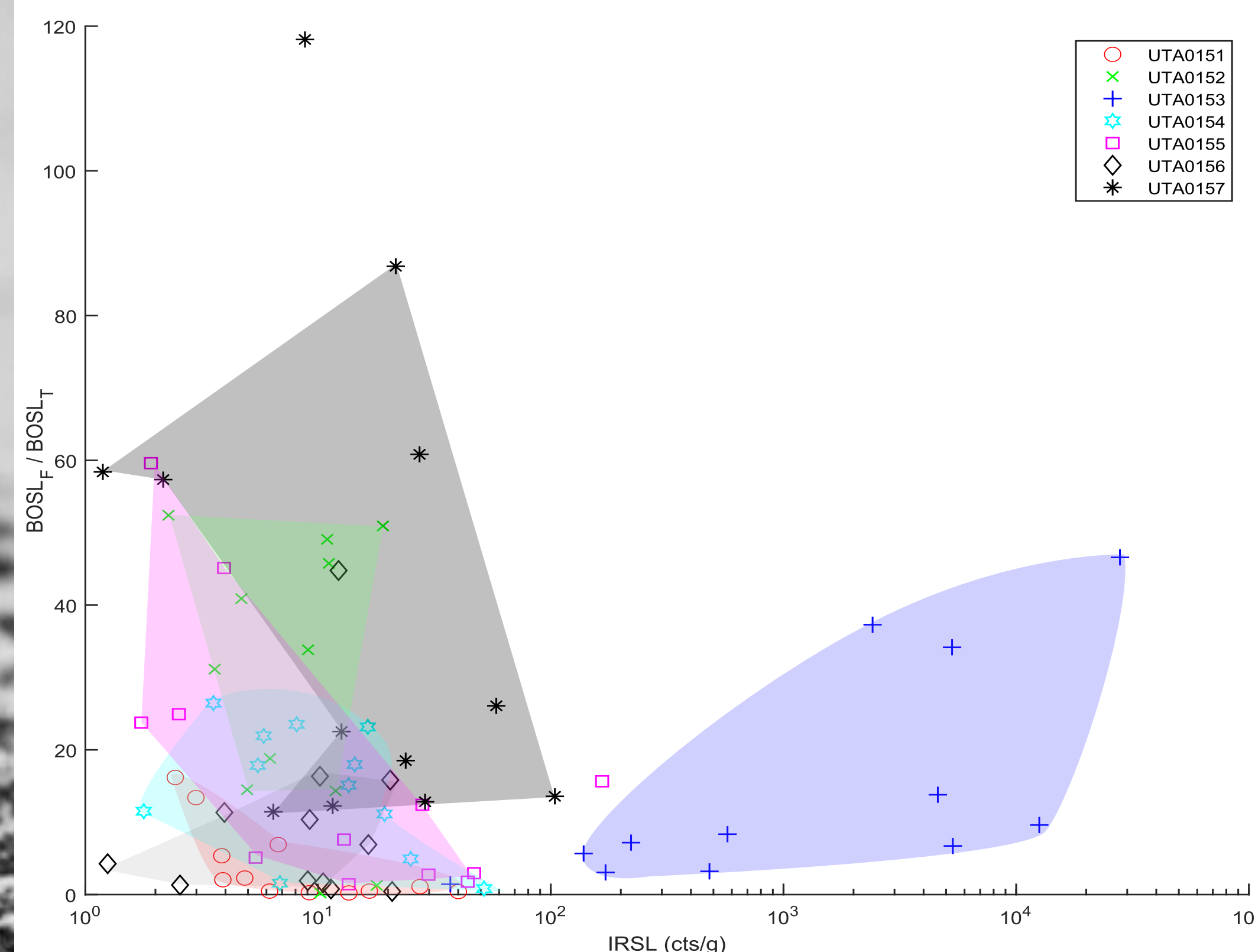
Figure 3. BSL and IRSI luminescence sensitivities in polymineral aliquots of riverbed sands. (brighter quartz = higher values) plotted against the total infrared stimulated luminescence intensity, (brighter feldspar = higher values).
