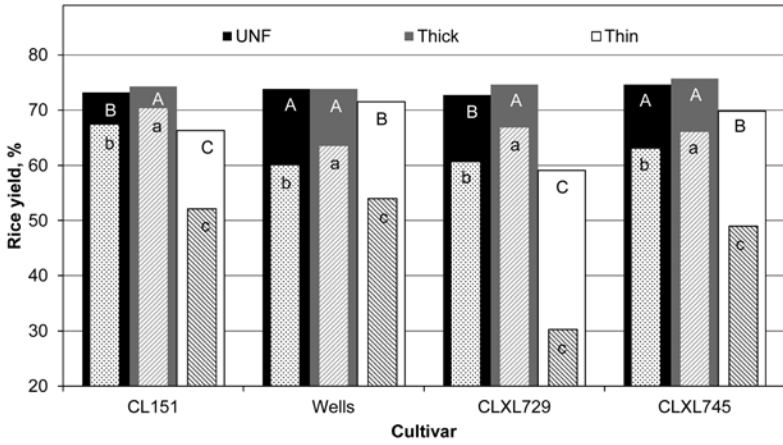
Fig. 2. Rice yield [milled rice yield (MR Y) or head rice yield (HR Y); milling duration of 30 s] of thickness fractions, in response to thickness-grading of rough rice of four long-grain cultivars. Fractions comprise Thick (>0.079 inch), Thin (<0.079 inch), and unfractioned (UNF) rice. Solid bars indicate MR Y and inset, crosshatched bars indicate HR Y. Letters inset within each bar facilitate the comparison of means within a cultivar; uppercase letters are associated with MR Y, and lowercase letters with HR Y; means with the same letter were not significantly different ( P > 0.05 ).
