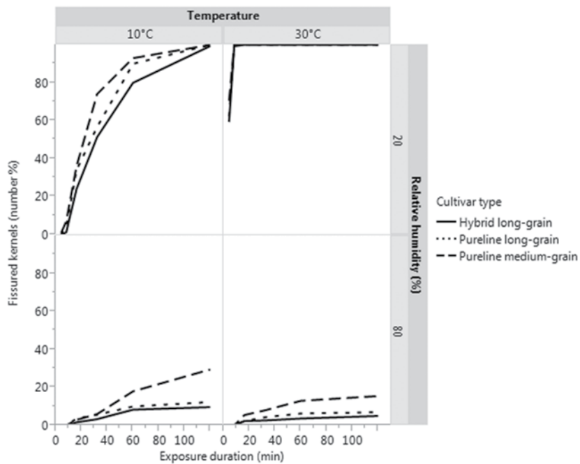
Fig. 4. Fissured kernel percentages at exposure durations of 4, 8, 16, 32, 60, and 120 min for the indicated cultivar lots when exposed to air at temperatures of 10 °C and 30 °C and relative humidities of 20% and 80%. The data are categorized into three cultivar groups: hybrid long-grain (CLXL729, CLXL745, and XL753), pure-line long-grain (CL151, Wells, and Cheniere), and pure-line medium-grain (CL261 and Jupiter). Curves are based on data representing the mean values of four replications.
