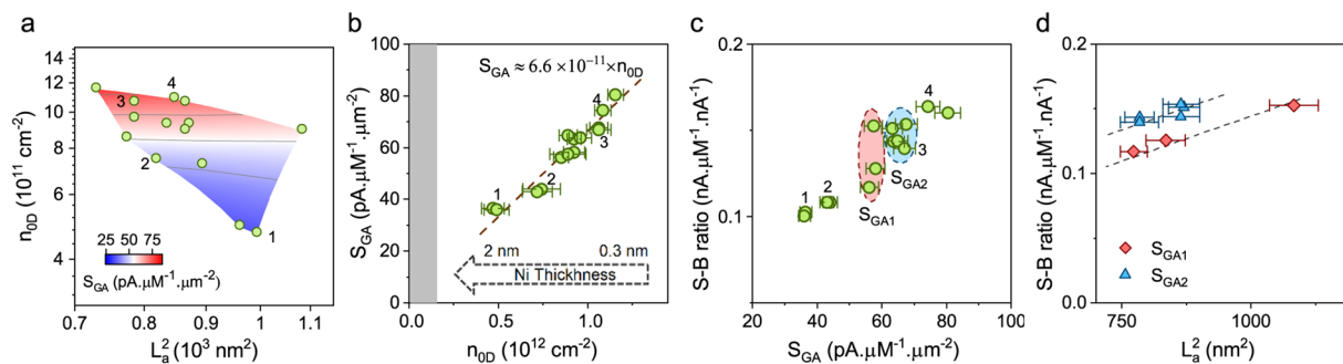
Figure 4. Effect of material structure on main sensor characteristics. (a) Contour plot of S_{GA} against n_{0D} and L_a^2 . (b) The plot of S_{GA} against n_{0D} , showing a linear trend. The grey shading represents the region where n_{0D} is below the detection limit of Raman. The error bars of S_{GA} are \pm 5\% and come from the uncertainties in calculations of the sensor area including the contribution of the surface roughness. (c) Scatter plot of S-B ratio against S_{GA} . The data show two sensor groups (denoted as S_{GA1} and S_{GA2} ), where sensors within each group had similar S_{GA} but different S-B ratio. (d) The monotonic increase of the S-B ratio with L_a^2 for these two sensor groups suggests the effect of L_a^2 on the background current. The dashed lines are guide for the eyes. The numbers next to the data points (1, 2, 3, 4) indicate the device names of four representative NG micro-sensors, which cover the entire range of measured S_{GA} and S-B ratio in our experiments. The FSCV characteristics of these sensors are shown in the Supplementary Information. The error bars of the S-B ratio are less than \pm 4\% .
