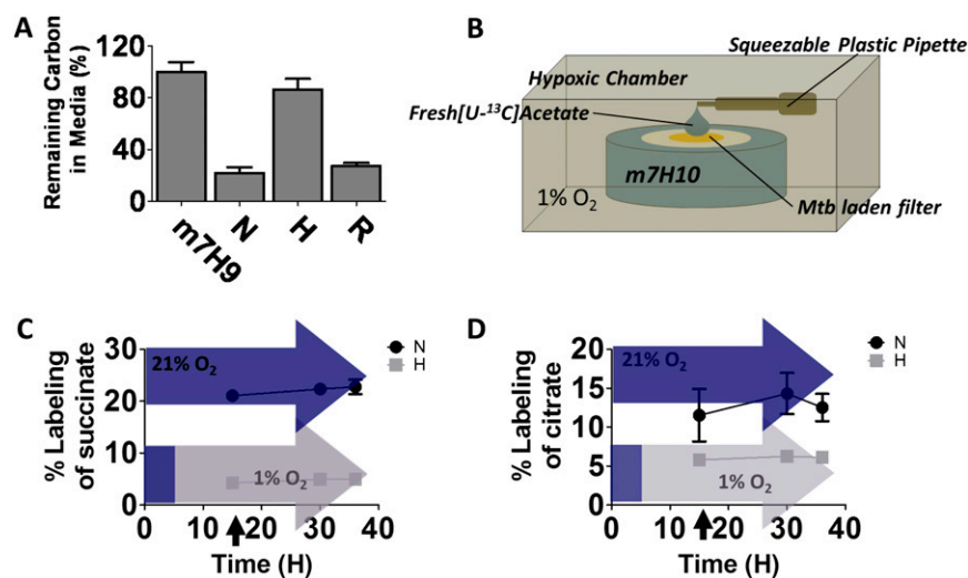
Fig. S2. Metabolically active but slowing of M. tuberculosis adaptive to 1% O 2 . (A) Relative depletion and/or consumption of extracellular acetate by M. tuberculosis incubated for 24 h at 21% O 2 (N), 1% O 2 (H), and at 21% O 2 following re-aeration of M. tuberculosis preincubated at 1% O 2 for 48 h (R). Uptake and/or consumption were reported by LC-MS-based measurements of remaining 13 C acetate content of extracellular media (as described in the main text and Materials and Methods using the device depicted in Fig. S7A) and expressed relative to media-only control samples [Middlebrook 7H9 (m7H9)]. (B–D) Bulk metabolic activity of putative tricarboxylic acid (TCA) cycle in M. tuberculosis at 1% O 2 was measured by using the device depicted in Fig. S2B. The hypoxic chambers used are flexible plastic bags that contain a squeezeable, plastic Pasteur pipette preloaded with fresh media containing 13 C-labeled carbon affixed to the roof of the bag, as depicted. Following conversion of a resazurin indicator inside the bag to white (indicative of 1% O 2 condition, which was achieved by 12 h after initiation of the catalytic reaction), fresh media containing 13 C carbon was released onto hypoxic M. tuberculosis by squeezing the preinserted pipette without breaking the hypoxic seal or causing the resazurin indicator to turn pink. The bulk metabolic activity of M. tuberculosis at either 1% O 2 or 21% O 2 was reported by isotopic labeling measurements of succinate (C) and citrate (D) following “pulsed” addition of fresh [U- 13 C] acetate-containing media to M. tuberculosis preadapted to 1% O 2 or 21% O 2 , at the time, as indicated by black arrows, when M. tuberculosis adapted to hypoxia entered metabolically stationary phase (Fig. S3). The large block arrows in C and D indicate the O 2 concentration in the environment where M. tuberculosis incubated.
