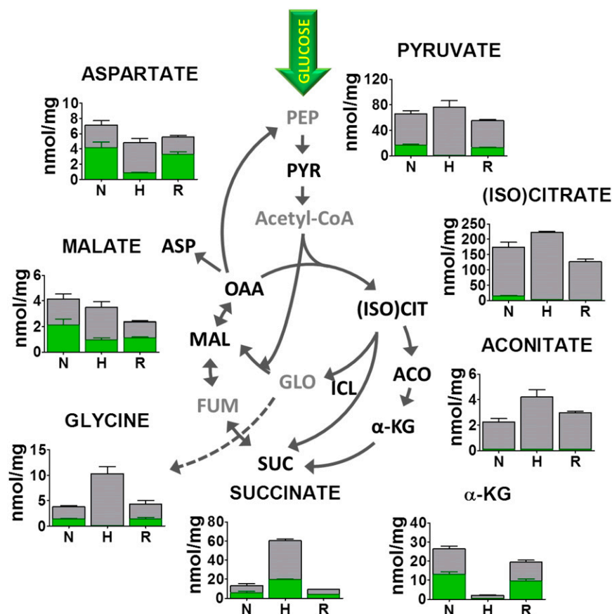
Fig. S5. Hypoxia-induced remodeling of M. tuberculosis TCA cycle activity when incubated with glucose as a defined carbon source. Intrabacterial pool sizes and isotopic labeling of TCA cycle-related intermediates in M. tuberculosis incubated in [U- 13 C] glucose-containing media for 24 h at 21% O 2 (N), 1% O 2 (H), and at 21% O 2 following reoxygenation of M. tuberculosis preincubated at 1% O 2 for 48 h (R). Total bar heights indicate the intrabacterial concentration; the green colored area of each bar denotes the extent of 13 C labeling achieved following transfer to [U- 13 C] glucose-containing media under the condition indicated. All values were the average of at least three experimental replicates in two independent experiments \pm SEM. Abbreviations are as in Fig. S4.
