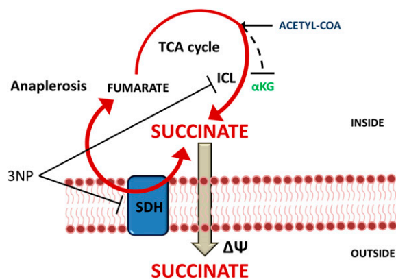
Fig. S9. Multifunctional essentiality of succinate during adaptation to 1% O 2 . Hypoxia triggers activation of isocitrate lyase activity, leading to an increase in succinate levels that can be used to support membrane potential, ATP synthesis, and anaplerosis during adaptation to, residence in, and recovery from hypoxia-induced quiescence. αKG, α-ketoglutarate; ΔΨ, membrane potential; ICL, isocitrate lyase; SDH, succinate dehydrogenase; 3NP, 3-nitropropionate.
