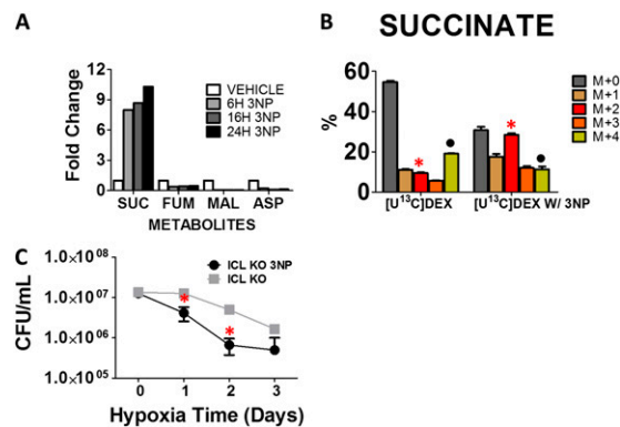
Fig. S8. Metabolic effect of 3-Nitropropionate (3NP) on M. tuberculosis metabolism and survival. (A) Metabolomic profiles of select TCA cycle intermediates in the presence of 200 μM 3NP at 21% O 2 for times as indicated. MAL, malate. (B) Isotopomeric profiles of succinate extracted from M. tuberculosis treated with 200 μM 3NP in [U- 13 C] glucose-containing media for 24 h at 21% O 2 . Red asterisks indicate 13 C 2 -labeled succinate; black circles indicate 13 C 4 -labeled succinate. (C) Viability of ΔICL KO following incubation at 1% O 2 in the absence or presence of 200 μM 3NP in 0.2% glucose-containing media. *P < 0.001 by ANOVA. All values were the average of at least three experimental replicates in two independent experiments ±SEM.
