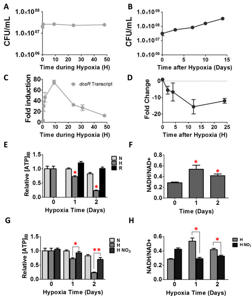
Fig. S1. Multimodal adaptation of Mycobacterium tuberculosis to 1% O 2 . (A) M. tuberculosis viability during adaptation to 1% O 2 reported by enumeration of colony forming units (CFUs) at indicated time points following transfer to 1% O 2 . (B) Reentry of M. tuberculosis adapted to 1% O 2 into cell cycle following re-aeration with 21% O 2 , as reported by CFU. (C) Time-dependent induction of dosR mRNA levels, a previously validated transcriptional marker of hypoxia (1), following transfer of M. tuberculosis to 1% O 2 . (D) Deinduction of dosR transcript levels, as reported by fold change relative to that measured at 24 h 1% O 2 . dosR mRNA levels were quantified by qRT-PCR, normalized to transcript levels of the housekeeping gene sigA , and expressed relative to those measured in M. tuberculosis incubated at 21% O 2 . (E) Relative intrabacterial ATP content of M. tuberculosis incubated for 24 h and 48 h at 21% O 2 (N), 1% O 2 (H), and following 24 h of re-aeration at 21% O 2 (R). (F) NADH/NAD ratio of M. tuberculosis incubated at 1% O 2 for 24 h and 48 h. Time 0 represents values measured at 21% O 2 . (G) The effect of presence of an alternate terminal electron acceptor (nitrate, NO 3 ) of the electron transport chain on hypoxic M. tuberculosis metabolism. Intrabacterial ATP content of M. tuberculosis incubated for 24 h at 21% O 2 (N), 1% O 2 (H), and 1% O 2 in the presence of 5 mM extracellular nitrate (H NO 3 ). (H) NADH/NAD ratio of M. tuberculosis incubated at 1% O 2 in the presence of 5 mM extracellular nitrate. Time 0 represents values measured at 21% O 2 . * P < 0.05 or *** P < 0.001. All values were the average of at least three experimental replicates in two independent experiments ±SEM.
