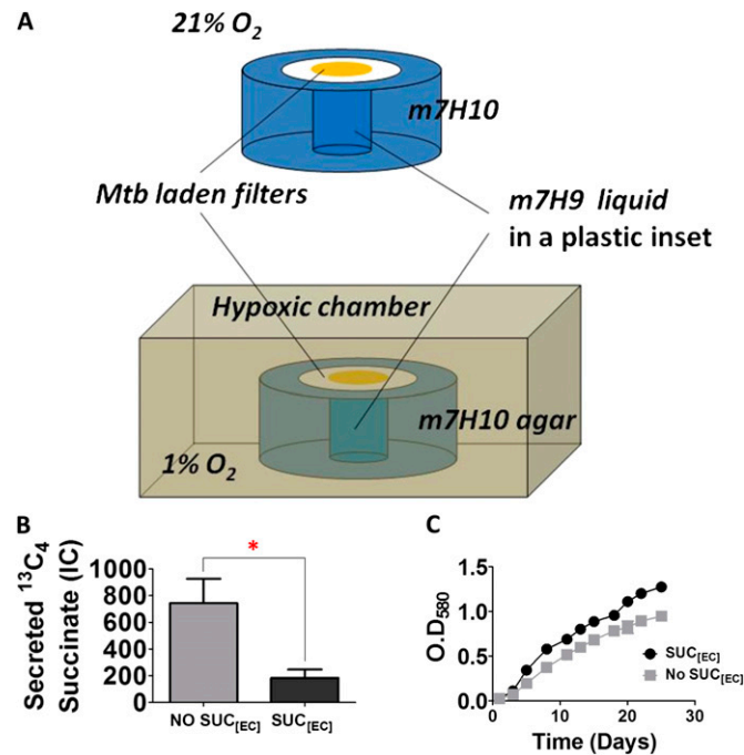
Fig. S7. The effect of succinate in extracellular media on M. tuberculosis metabolism. (A) Schematic diagram illustrating the device used to make timed start-stop measurements of secretion into the extracellular media which consists in a plastic inset containing chemically equivalent liquid media (m7H9) amenable to experimental sampling. (B) The effect of 2 mM succinate in extracellular medium on secretion of intracellular succinate from hypoxic (1% O 2 ) M. tuberculosis . Relative levels of secreted intracellular succinate measured using the device depicted in Fig. S7A with plates containing or lacking 2 mM unlabeled extracellular succinate. To distinguish secreted intracellularly synthesized succinate from exogenously supplied (unlabeled) extracellular succinate, M. tuberculosis -laden filters were preincubated on m7H10 containing [U- 13 C] acetate for 2 d to label intracellular succinate within bacilli with 13 C. M. tuberculosis -laden filters were then transferred to the devices shown in Fig. S7A and incubated for 20 h at 1% O 2 . The amount of succinate secretion from M. tuberculosis bacilli during incubation in the presence or absence of unlabeled extracellular succinate was reported by the ion count intensities (IC) of 13 C 4 succinate isotopologue using LC-MS. The addition of unlabeled extracellular succinate thus efficiently prevented secretion of intracellular succinate from hypoxic M. tuberculosis adapted to 1% O 2 (compare bar heights shown Left and Right). *P < 0.001 by ANOVA. All values were the average of at least three experimental replicates in two independent experiments ±SEM. (C) The effect of the same concentration of extracellular succinate on M. tuberculosis growth under aerobic conditions (in the presence of 0.2% acetate).
