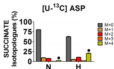
Fig. S6. Isotopomeric profiles of succinate extracted from M. tuberculosis treated with [U- 13 C] aspartate in the presence of acetate in media for 24 h at either 21% O 2 (N) or 1% O 2 (H). M+0, unlabeled; M+1, singly 13 C labeled; M+2, doubly 13 C labeled succinate, and so on. Black circles indicate 13 C 4 -labeled succinate (predominant incorporation of 13 C 4 is consistent with en bloc incorporation and biosynthesis of succinate via reductive TCA cycle activity).
