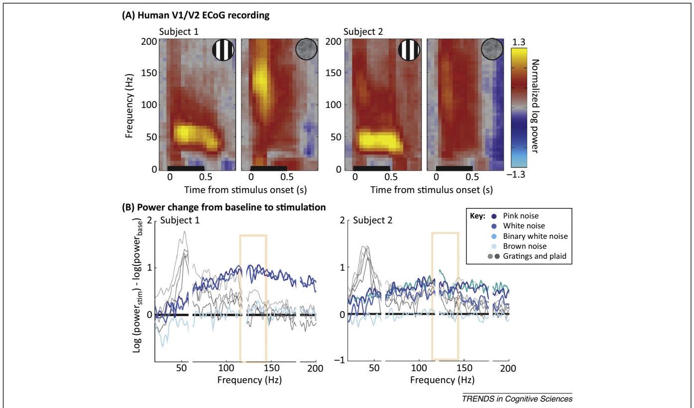
Figure 1. Stimulus effects on gamma oscillations. (A) Power changes from baseline from ECoG recordings in human V1/V2, plotted as a function of time and frequency. Grating stimuli elicit large, sustained gamma oscillations around 50 Hz. In higher frequencies (above 80 Hz), a transient response is present. Noise stimuli elicit a different pattern of responses. Narrowband gamma oscillations from 30 to 80 Hz are not evident. In higher frequencies (above 80 Hz), both a large transient and a smaller sustained response are present. Adapted from Figure 1 of [3] and reproduced with permission from Oxford University Press. (B) Plots of spectral power change from baseline for several stimuli. The Brunet et al. article [5] argues that the power changes from baseline show a convincing spectral peak around 130 Hz for noise patterns. This area is highlighted in yellow. Data at 60 Hz, 120 Hz, and 180 Hz are masked due to contamination from electrical line noise. Adapted from Figure 2 of [3] and reproduced with permission from Oxford University Press.
