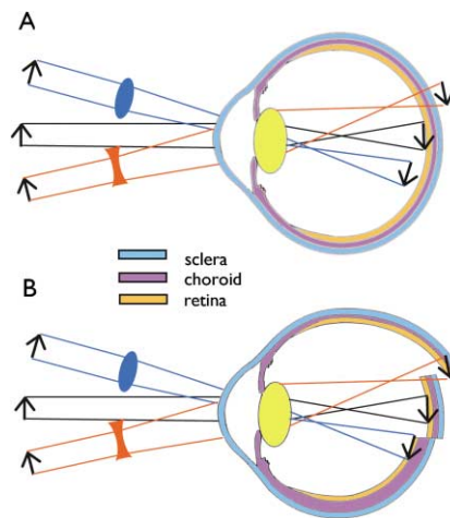
Figure 2. Ocular Compensation for Lens-Induced Defocus (A) A positive lens (blue, convex) causes the image to form in front of the retina (myopic defocus), whereas a negative lens (red, concave) pushes the image plane behind the retina (hyperopic defocus). With no lens (black rays), the image of a distant object is focused on the retina. (B) The eye compensates for positive lenses by slowing its rate of elongation and by thickening the choroid, pushing the retina forward toward the image plane. It compensates for negative lenses by increasing the rate of elongation and thinning the choroid, pulling the retina back toward the image plane. The emmetropic eye is intermediate in length and in choroid thickness.
