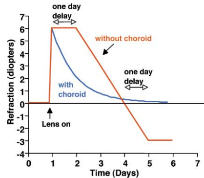
Figure 5. Dynamics of Spectacle-Lens Compensation
