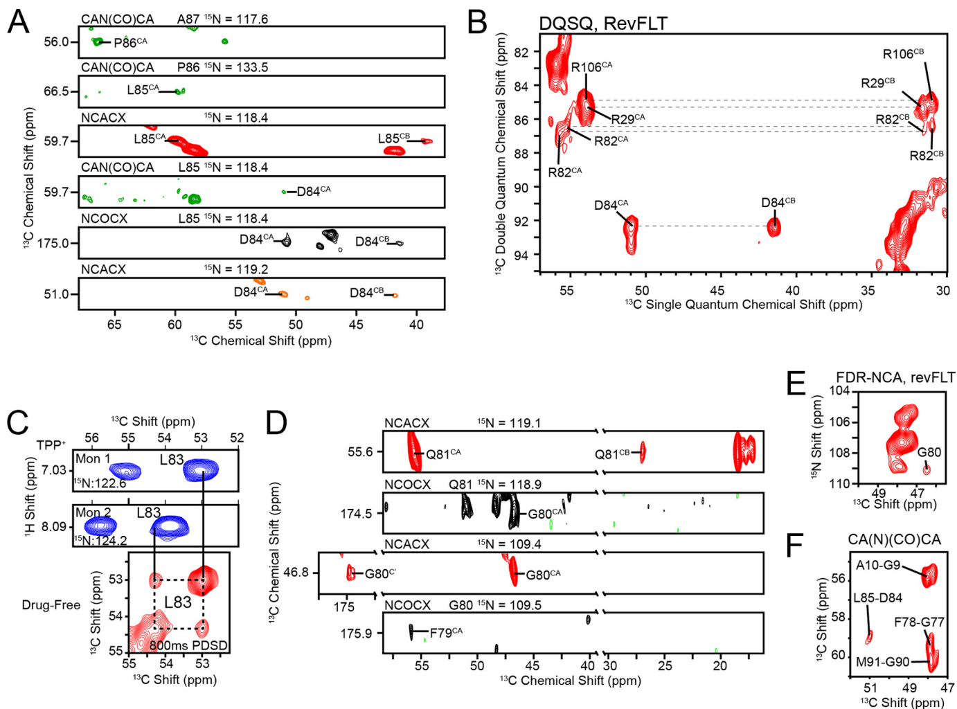
FIGURE 3. Spectroscopic characterization of the loop connecting TM3 and TM4 in the drug-free state in DMPC-liposomes. A , the backbone resonances for [U-^{13}C, ^{15}N] EmrE were assigned with MAS-SSNMR using a backbone walk with CAN(CO)CA (green), NCACX (red/orange), and NCOCX (black) experiments. Note that the orange NCACX (Asp 84 ) was collected with revWIY-labeled EmrE. B , DQSQ experiment with revFLT shows the arginine residues clustered around 55 ppm. Unlike Arg 29 and Arg 106 , Arg 82 is split into two distinct peaks, which results in a weaker signal overall. The assignment for Arg 82 is also in good agreement with data collected from solution NMR (Fig. 4). C , similarity of chemical shifts in the TPP + -bound form from solution NMR (blue) are directly transferable to spectra collected in the drug-free form with MAS-SSNMR, which provided the assignment for Leu 83 in an 800-ms PDSO experiment on [2-^{13}C, ^{15}N] Leu EmrE. D , Gln 81 , Gly 80 , and Phe 79 are visible in NCACX and NCOCX spectra collected at 750 MHz ( 1 H frequency) with [U-^{13}C, ^{15}N] EmrE in 3/1 DMPC/DMPG and are in good agreement with data from solution NMR. E , the FDR-NCA with revFLT served as a spectroscopic filter that highlighted residues i + i relative to the reverse labeled amino acids and allowed for the assignment of Gly 80 (28). F , a two-dimensional CA(N)(CO)CA with [U-^{13}C, ^{15}N] EmrE was used to assign Gly 77 and Phe 78 .
