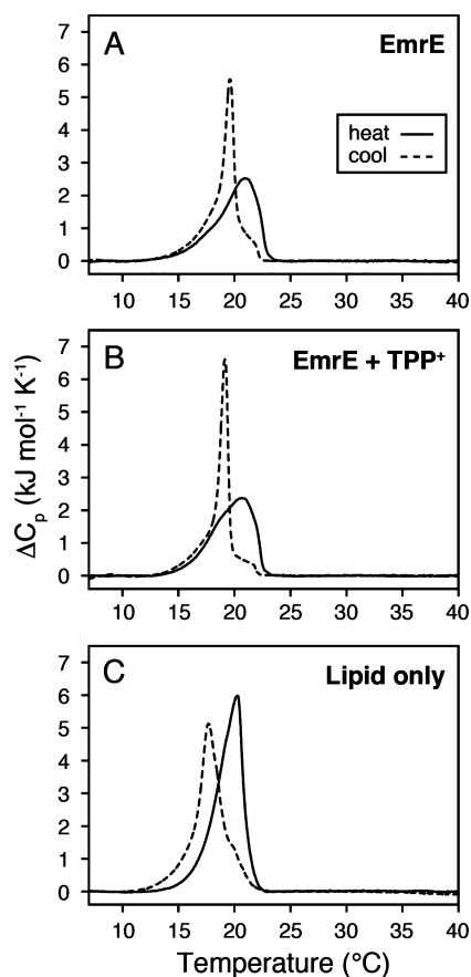
Figure 3. DSC thermogram data for 3/1 POPE/POPG bilayers in the presence of protonated-EmrE (A), TPP + -bound EmrE (B), and lipid-only (C). The samples containing EmrE used a lipid/protein molar ratio of 100/1. The heating (solid lines) and cooling curves (dotted lines) are shown for each sample. The line widths corresponding to EmrE in the absence and presence of TPP + show similar profiles when comparing heating or cooling curves, which is consistent with 16:0-PC data in Figure 1D. However, due to the observed thermal hysteresis for the lipid-only POPE/POPG mixture, only qualitative conclusions can be drawn regarding the effect of TPP + binding to EmrE on the phase transitions.
