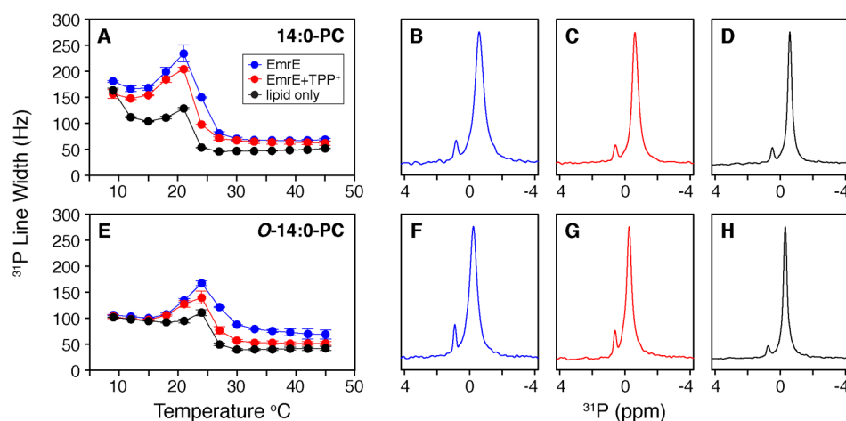
Figure 4. ^{31}\text{P} line widths from a single pulse MAS experiment for EmrE embedded within 14:0-PC (A) and O-14:0-PC bilayers (E). The blue and red points correspond to EmrE in the absence and presence of TPP ^{+} , respectively. The black points correspond to the lipid-only samples. Data reflect the average of two separate trials where the error bars represent the standard deviation of these data sets. The ^{31}\text{P} line width vs temperature plots for each trial are shown in Figure S3. Representative ^{31}\text{P} spectra are shown at a temperature of 23 ^{\circ}\text{C} for 14:0-PC in the absence (B) and presence of TPP ^{+} (C) and lipid-only (D). The same is shown at 27 ^{\circ}\text{C} for O-14:0-PC in the absence (F) and presence of TPP ^{+} (G) and lipid-only (H). In both lipid compositions, there is a reduction in the ^{31}\text{P} line width when EmrE is bound with TPP ^{+} . Note that the small peak around \sim 1 ppm is the signal from the phosphate buffer used to prepare the samples.
