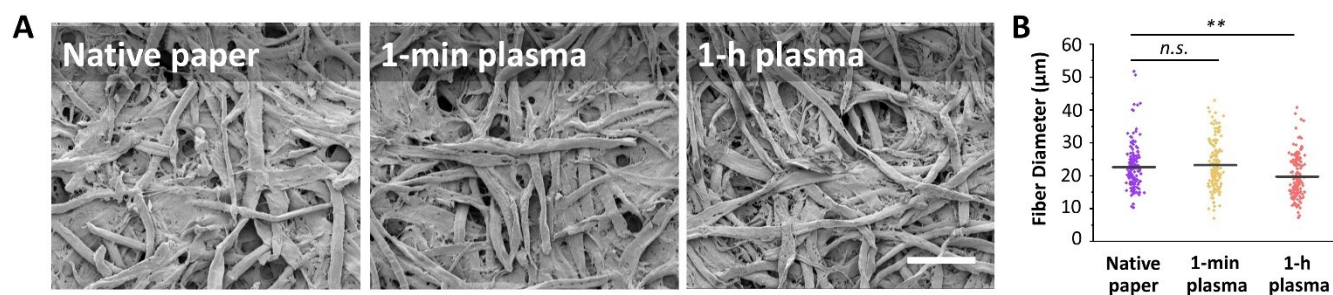
Fig. S1 Effect of air plasma treatment on microstructure of paper fibers. (A) SEM images show the surface characteristic of native (untreated) and 1-min and 1-h plasma-treated paper fibers. Exposure of one hour caused significant reduction in fiber diameters compared to exposure of one minute and untreated fibers. The scale bar is 150 μm. (B) Diameter distribution of paper fibers as measured for native paper and after 1-min and 1-h plasma exposures. n.s.: not significant and **: significant at P < 0.05 using two-sided student's t-test.
