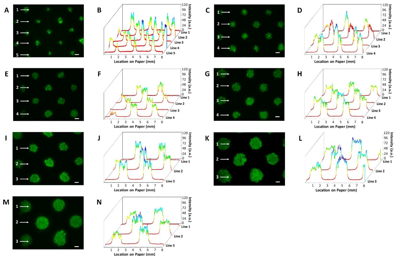
Fig. S2 Fluorescein characterization of hydrophilic microspots created using 3D printed masks with circular through-holes of different diameters. Fluorescence and 3D plots show fluorescence images of patterned microspots and the intensity across lines of patterns with hole diameters of (A-B) 400 \mu\text{m} , (C-D) 500 \mu\text{m} , (E-F) 600 \mu\text{m} , (G-H) 700 \mu\text{m} , (I-J) 800 \mu\text{m} , (K-L) 900 \mu\text{m} , and (M-N) 1000 \mu\text{m} . The scale bars are 500 \mu\text{m} .
