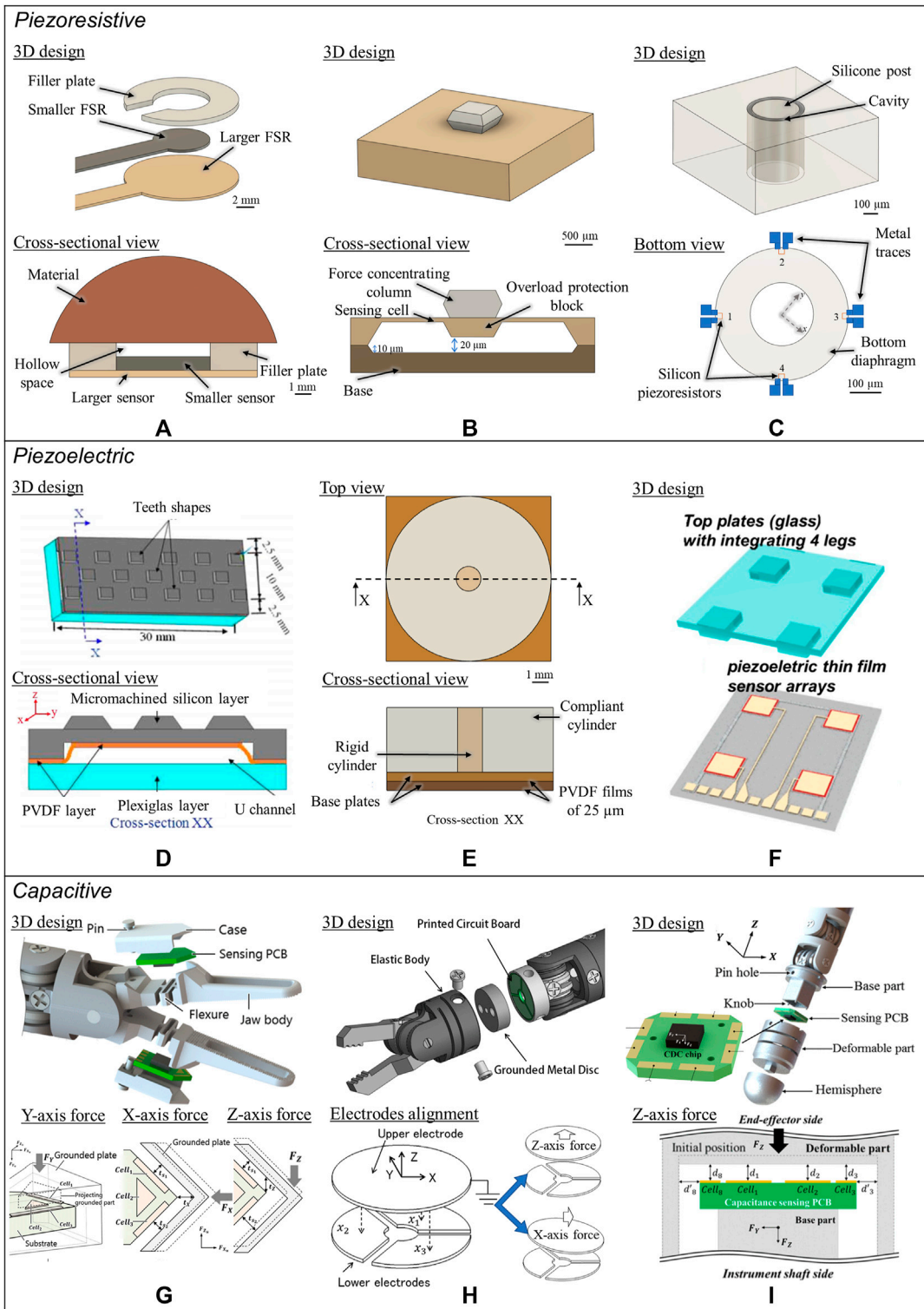
FIGURE 2 | Electrical-based tactile sensors for MIS. (A–C) Piezoresistive tactile sensing. (A) Schematic and cross-sectional view of the piezoresistive tactile sensor consisting of two circular force sensing resistors with different diameters and one plastic filler plate, which can differentiate between the hardness of other types of elastomers (Kalantari et al., 2010). (B) Illustration of mechanical structure and a cross-sectional view for the individual three-dimensional force sensing cell of the tactile sensor (Mei et al., 2000). (C) 3D illustration and backside view of the bioinspired piezoresistive tactile sensor consisting of a silicone post on top of a bottom diaphragm with strain gauges (Hu et al., 2010). (D–F) Piezoelectric tactile sensing. (D) Schematic showing the structure and cross-sectional view of PVDF-based piezoelectric tactile sensor composed of three layers: a double-sided micromachined silicon plate, a PVDF film, and a Plexiglas support layer (Qasaimeh et al., 2008a). © (Continued)
