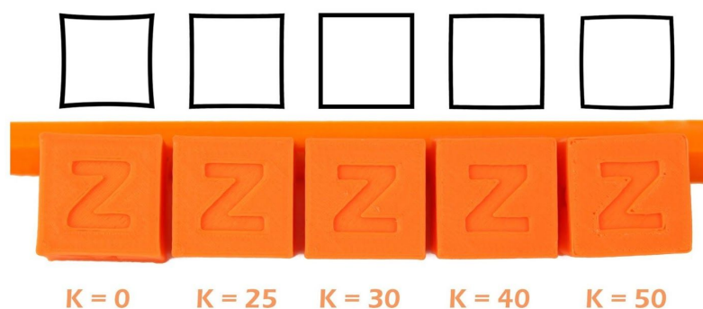
Pict. 25 - How K value affects the print
