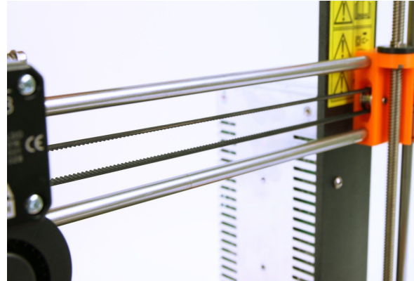
Pict. 49 - A properly-tightened X-axis belt
