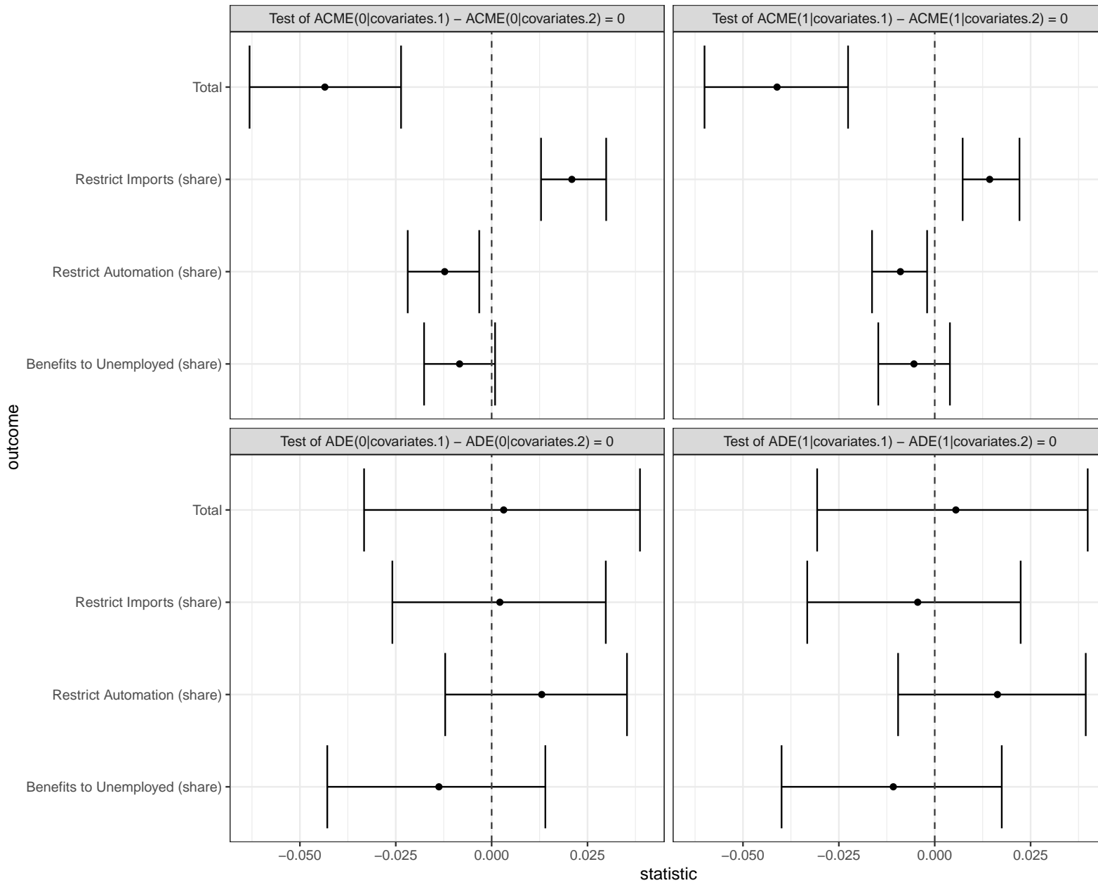
Figure 19: The ACME tests (comparing the ACME when quantile = 1 with ACME when quantile = 8) demonstrate evidence that nationalism moderates the mediated effect of quality on every variable except benefits to unemployed. I'm puzzled by the conflicting signs but otherwise I think this shows strong evidence.
