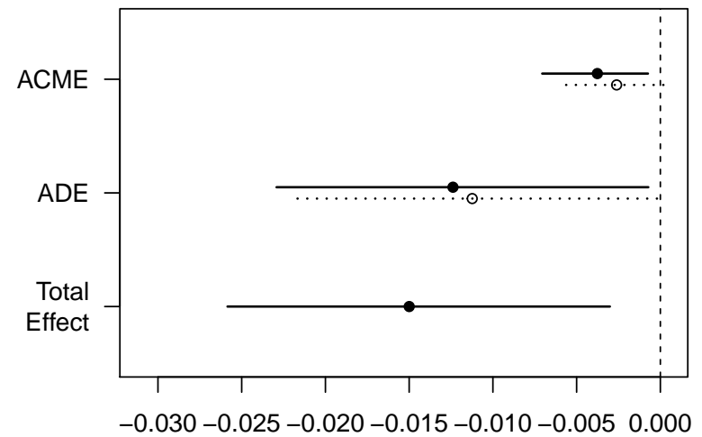
Figure 18: The mediation analysis suggests that nationalism has a strong negative effect on benefits to unemployed, both directly and through the channel of perceived quality declines. All variables show a conditional effect of nationalism going through the quality variable. The effect on wanting to restrict imports seems odd but the rest seem completely reasonable.
