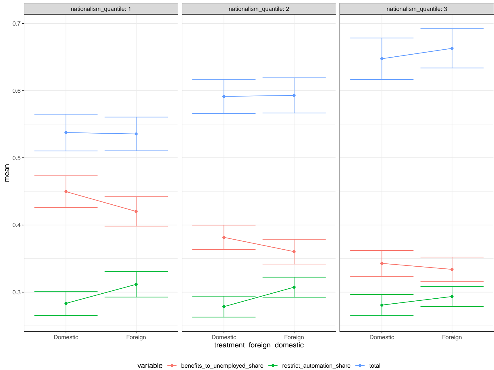
Figure 15: Treatment effect of foreignness on all variables of interest by quantile of nationalism_average_response, limited to automation only.
