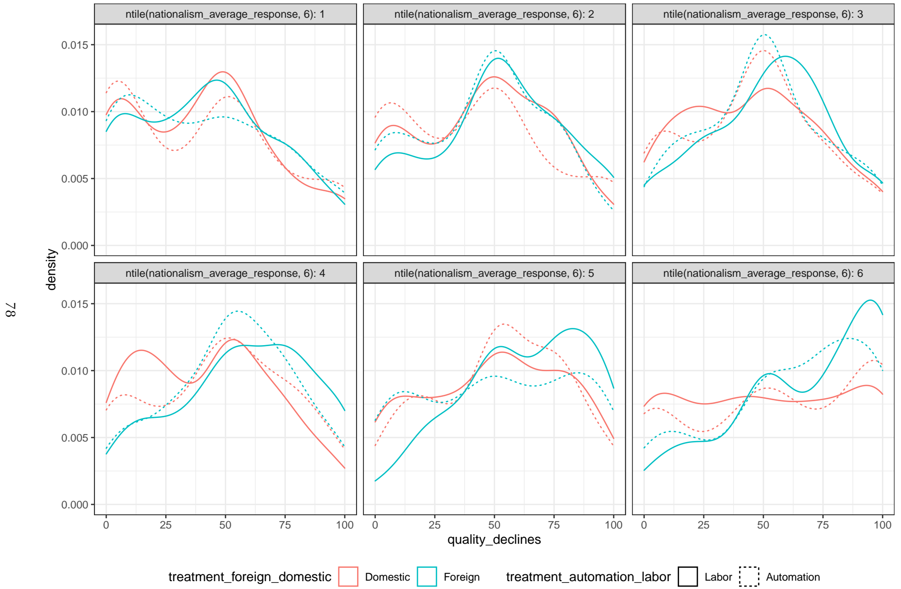
Figure 17: The effect is strongly mediated by nationalism
