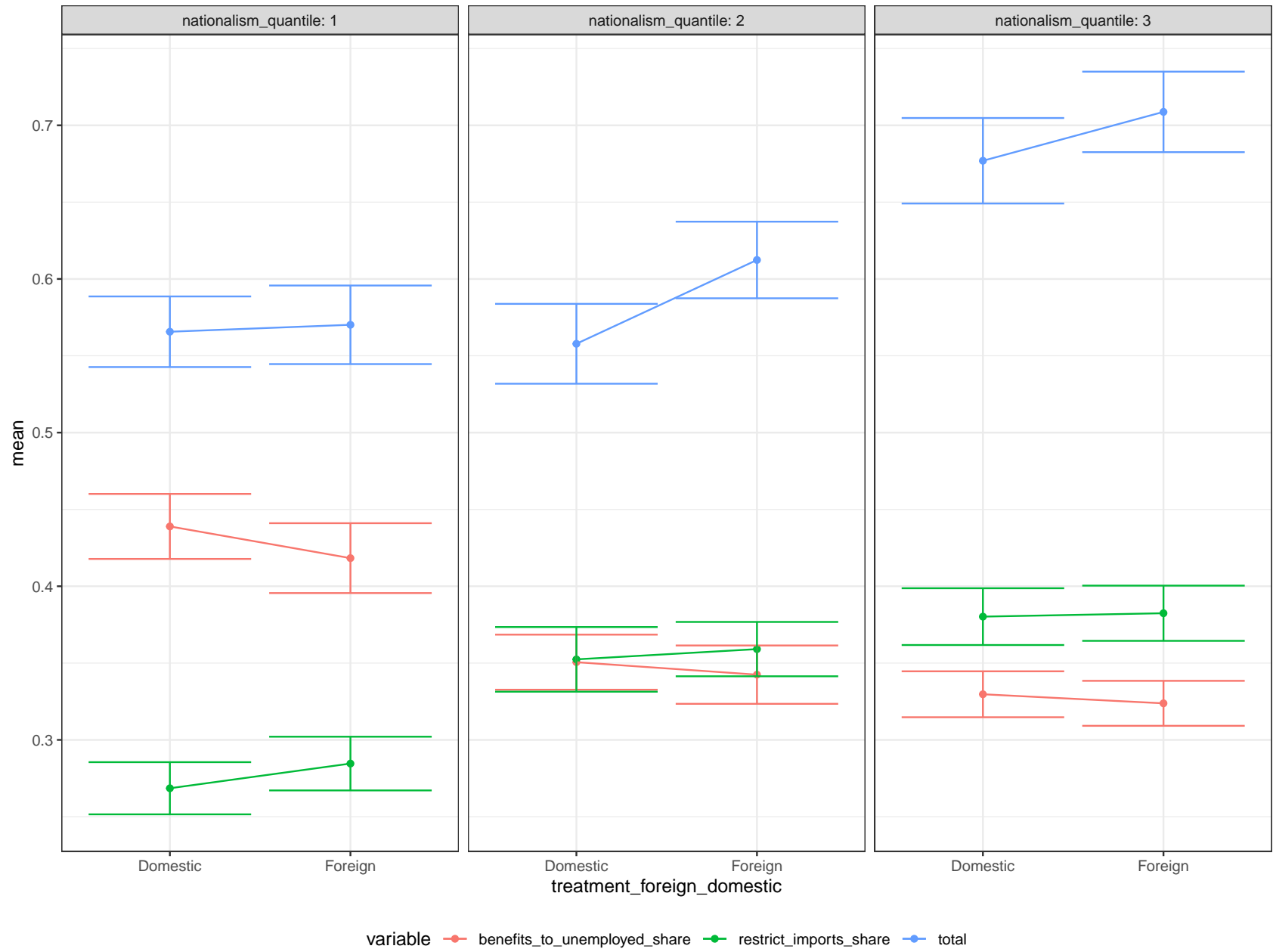
Figure 14: Treatment effect of foreignness on all variables of interest by quantile of nationalism_average_response, limited to labor only
