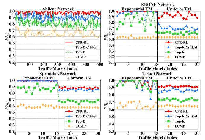
Fig. 5: Comparison of load balancing performance in the four networks on each test traffic matrix.
