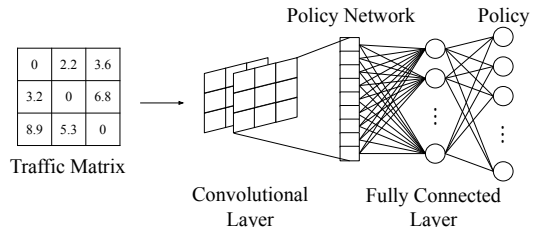
Fig. 2: Policy network architecture.
