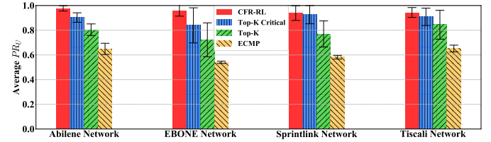
Fig. 4: Comparison of average load balancing performance ratio where error bars span \pm one standard deviation from the average on the entire test set of the four networks.
