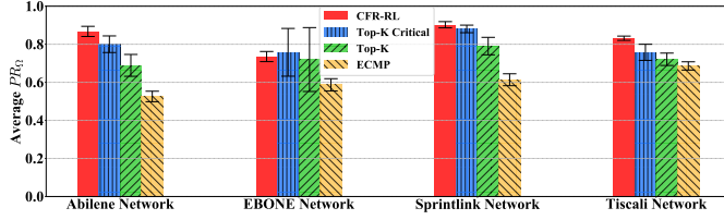
Fig. 6: Comparison of average end-to-end delay performance ratio where error bars span \pm one standard deviation from the average on the entire test set of the four networks.
