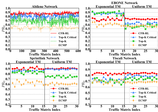
Fig. 7: Comparison of end-to-end delay performance in the four networks on each test traffic matrix.
