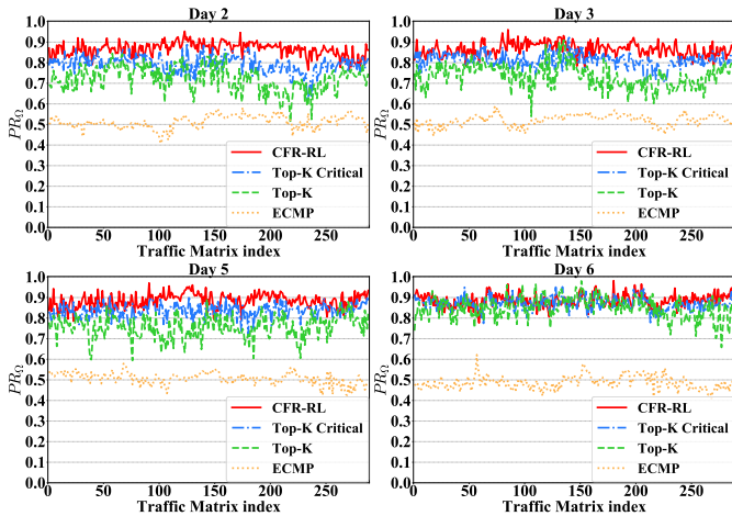
Fig. 11: Comparison of end-to-end delay performance ratio with the traffic matrices from Tuesday, Wednesday, Friday and Saturday in week 2.
