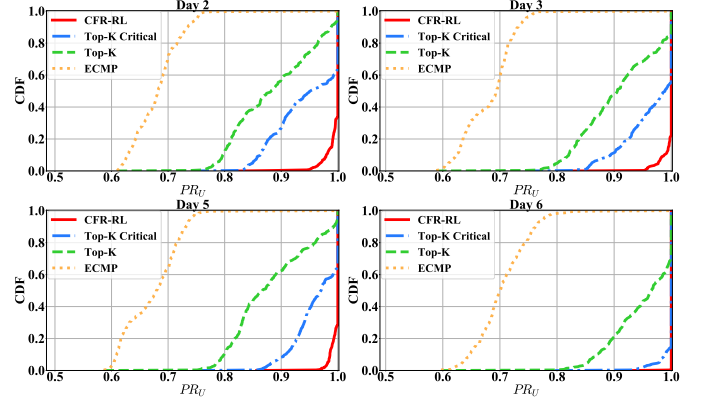
Fig. 8: Comparison of load balancing performance ratio in CDF with the traffic matrices from Tuesday, Wednesday, Friday and Saturday in week 2.
