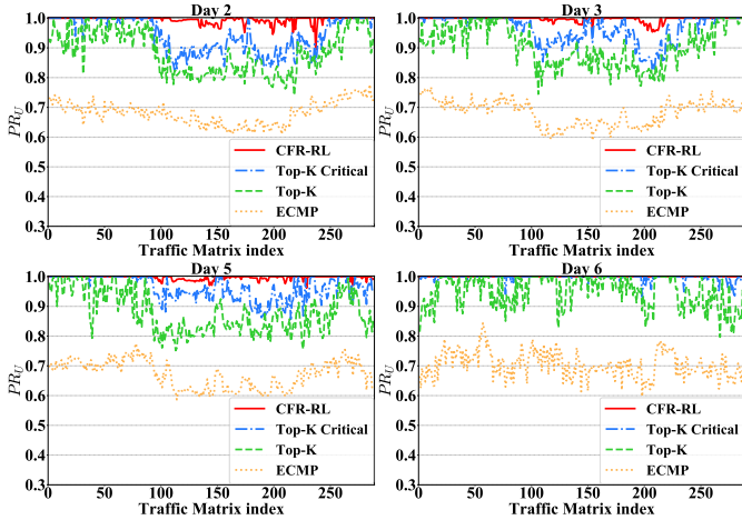
Fig. 10: Comparison of load balancing performance ratio with the traffic matrices from Tuesday, Wednesday, Friday and Saturday in week 2.
