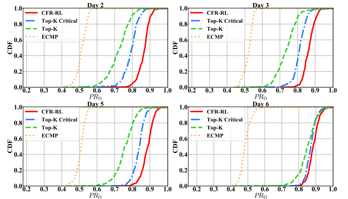
Fig. 9: Comparison of end-to-end delay performance ratio in CDF with the traffic matrices from Tuesday, Wednesday, Friday and Saturday in week 2.
